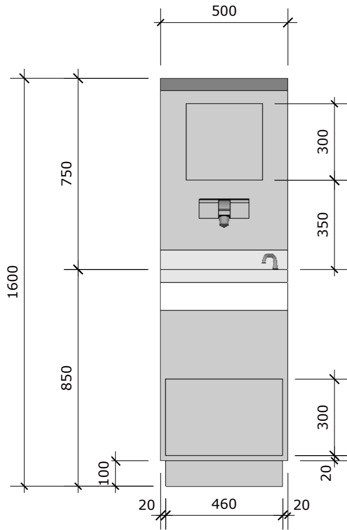
front elevation
