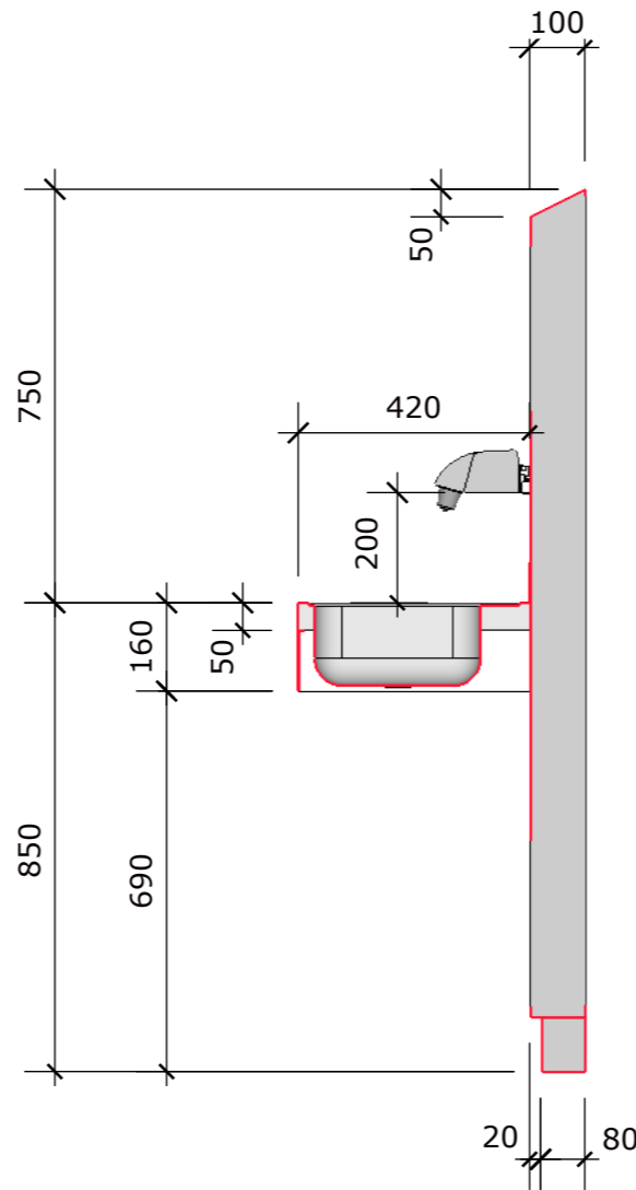
section thru
