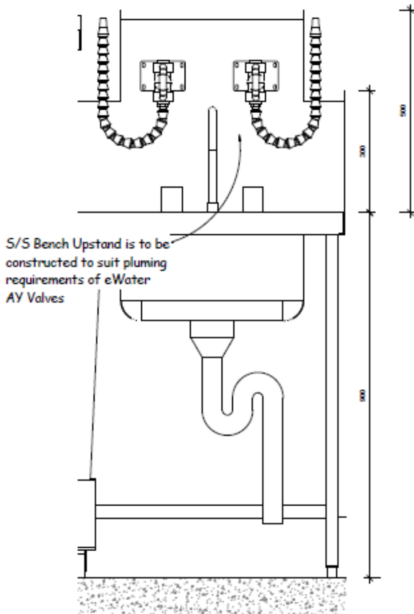
eWater mounting on Extended Bench Upstand Scale 1:5 @ A1
